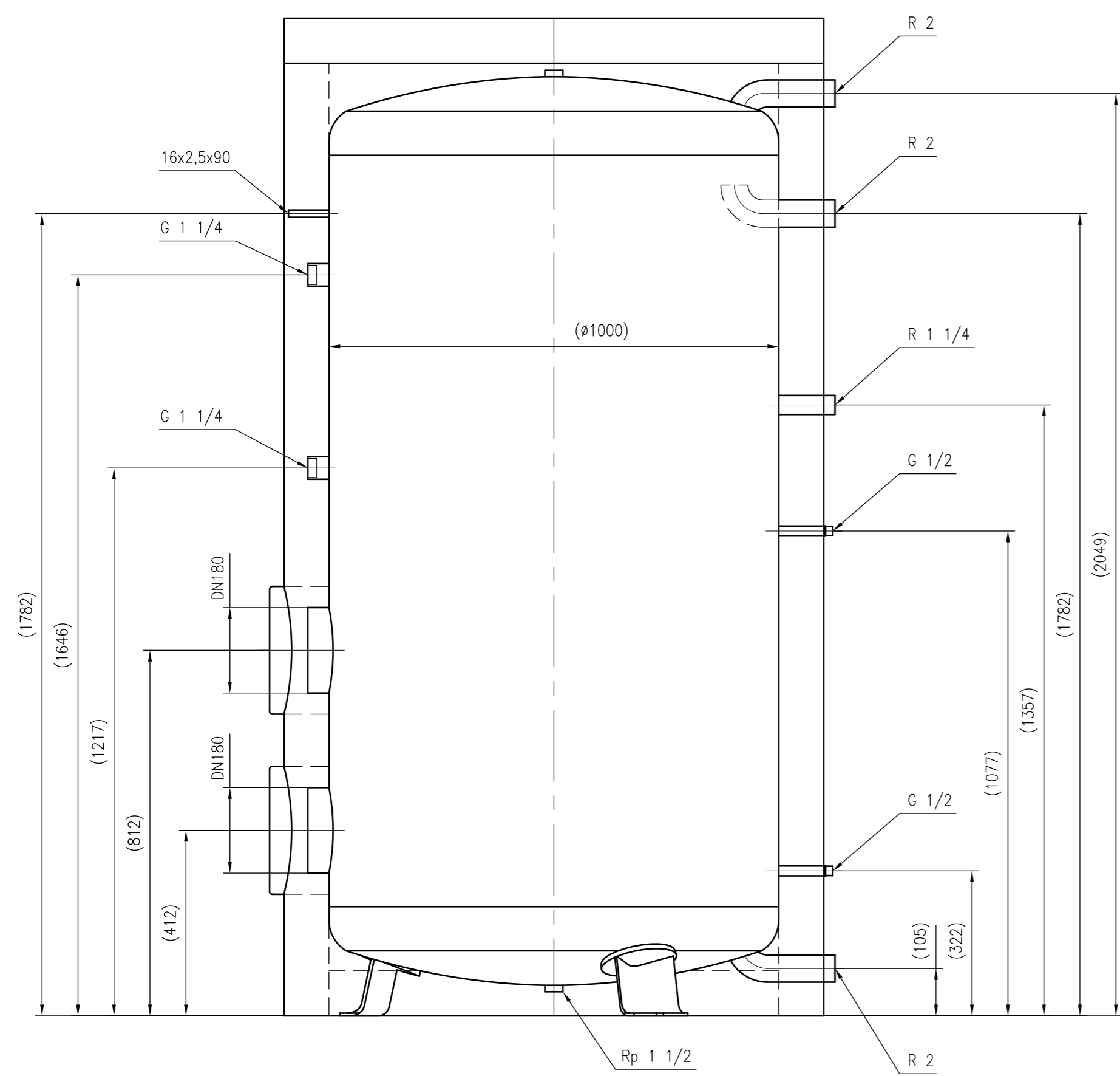
Side view
