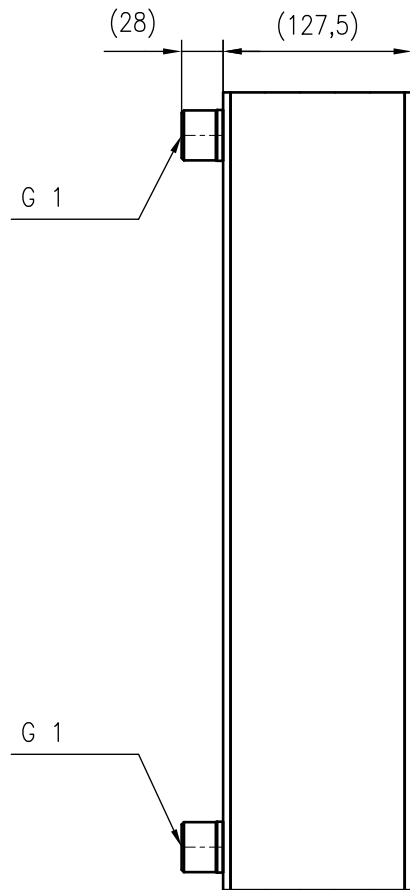
Side view
