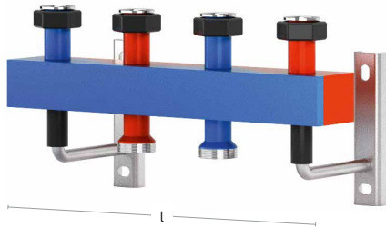
Small manifolds 80/60
