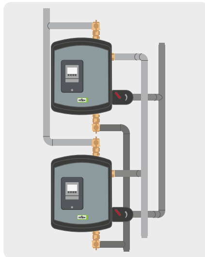
Vertical cascade pipework for two Reflex Hydroflow M
