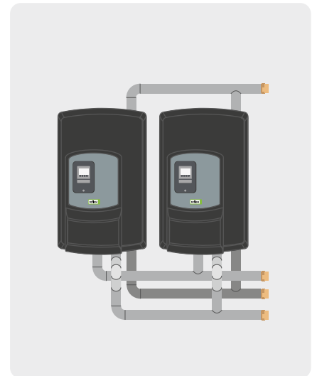
Horizontal cascade pipework to the right for two Reflex Hydroflow L
