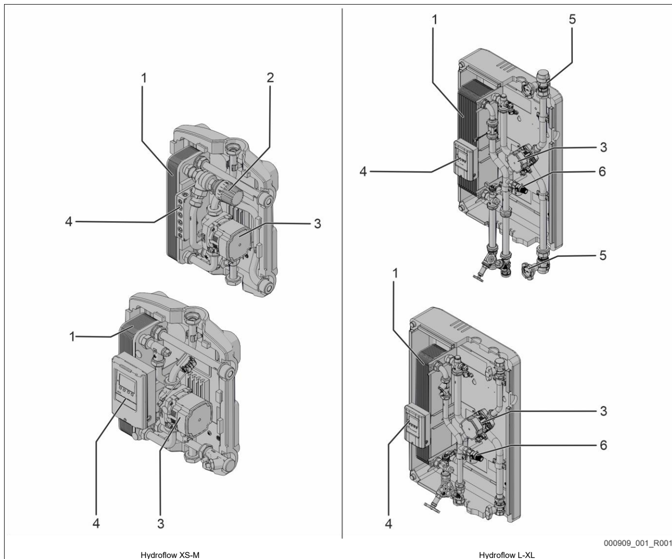
Hydroflow XS-M
